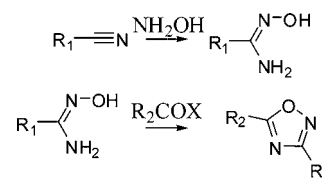
Scheme 2. General preparation method for 1,2,4-oxadiazoles
