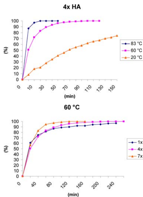
Figure 1. Reaction of benzonitrile (1a) in batch.
