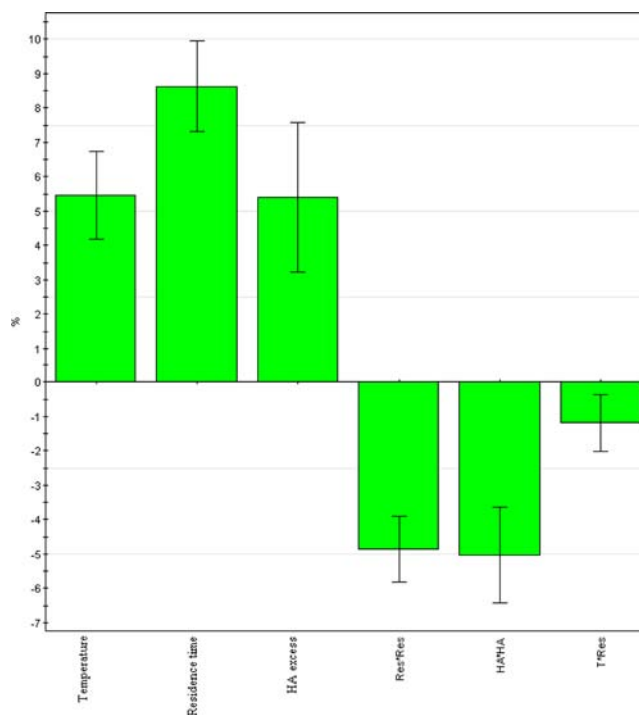
Figure 2. Coefficient plot of benzamidoxime formation.
