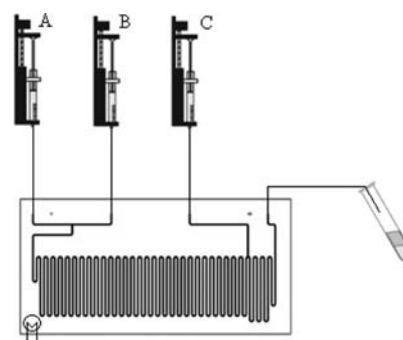
Figure 4. Labtrix S1 microreactor (10 \mu L) 30 A: nitrile compound in solvent, B: HA, C: quenching by solvent.
