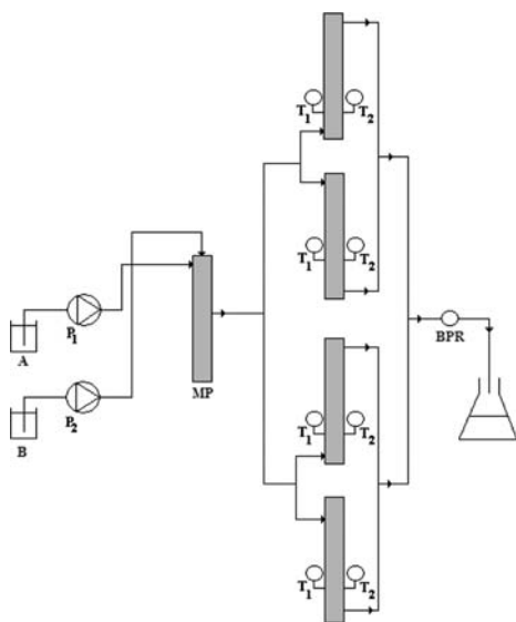
Figure 6. Corning LF reactor with four plates. 31 (A) Nitrile compound in solvent. (B) HA, MP: mixing plate. BPR: back pressure regulator.
