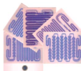
Figure 5. Corning reactorplates. 33,34
